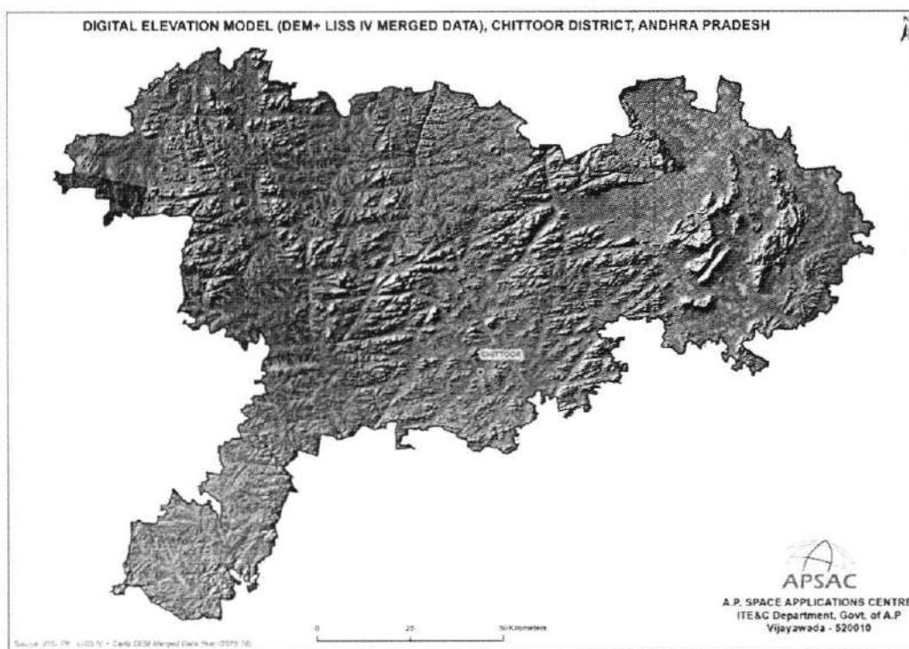
Fig.12 Digital Elevation Map Of Chittoor District,A.P
