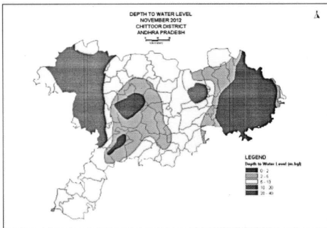
Fig.25. Post monsoon Water levels of Chittoor District.A.P
