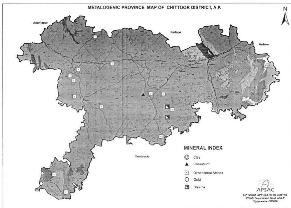
Fig 20: Metallogenic province Map of chittoor district, A.P
