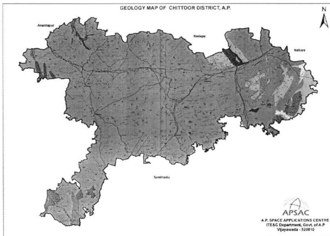
Fig 18: Geology Map of Chittoor District, A.P
