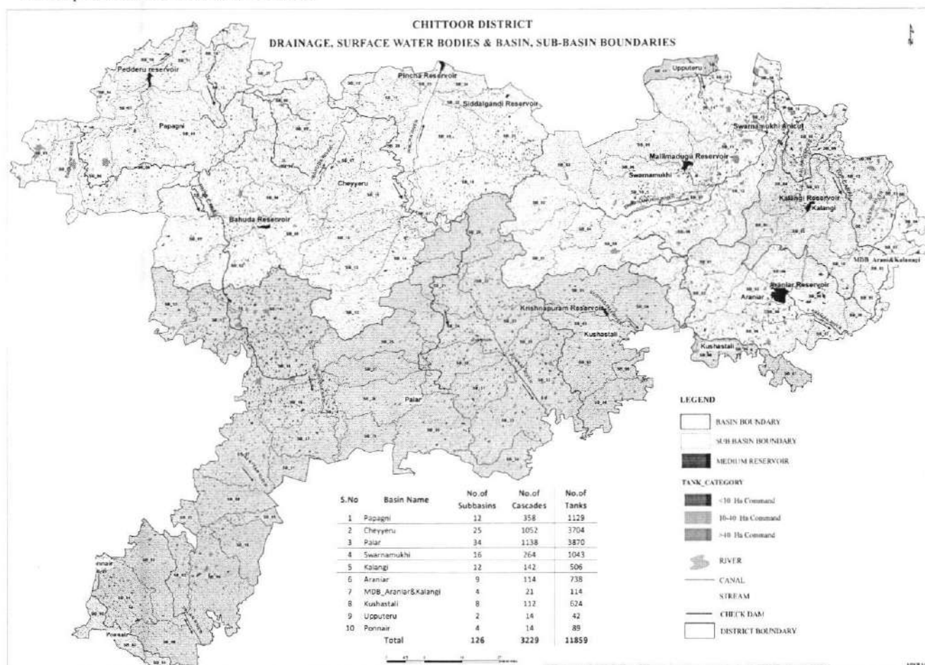
Fig.17. Drainage and surface water bodies, basin boundaries
