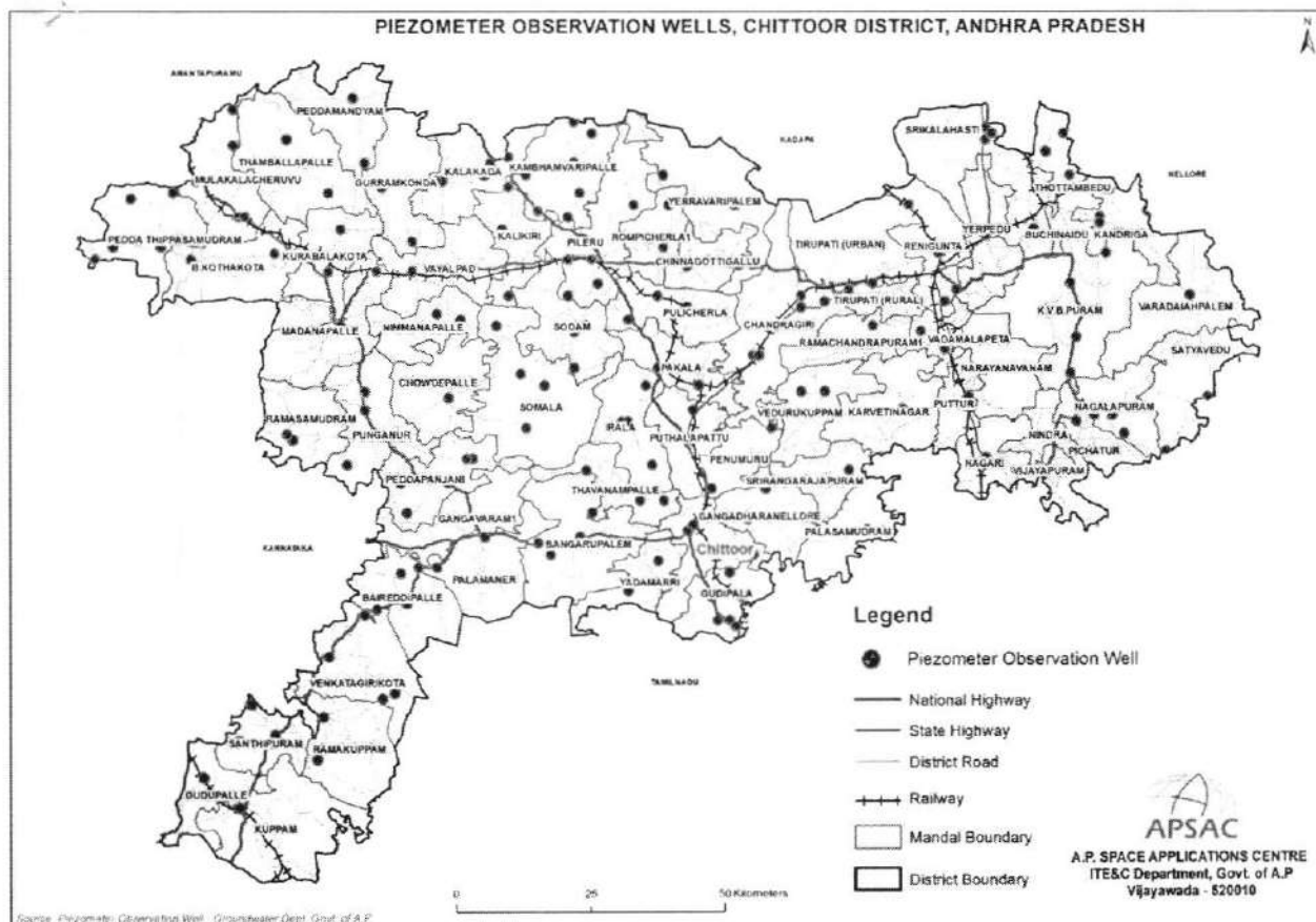
Fig 26: Piezometric observation well Map of chittoor district, A.P
