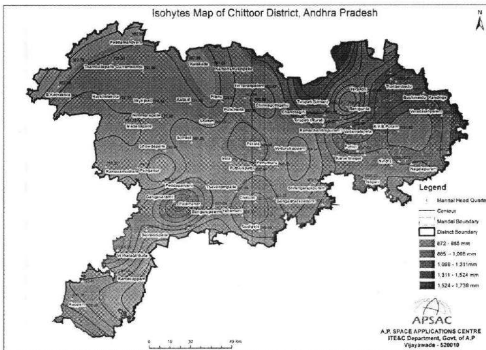
Fig.5.Rainfall distribution Chittoor District, A.P
