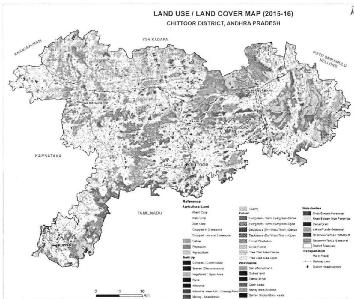
Fig.9. land use / land cover map of Chittoor District 2015- 2016
