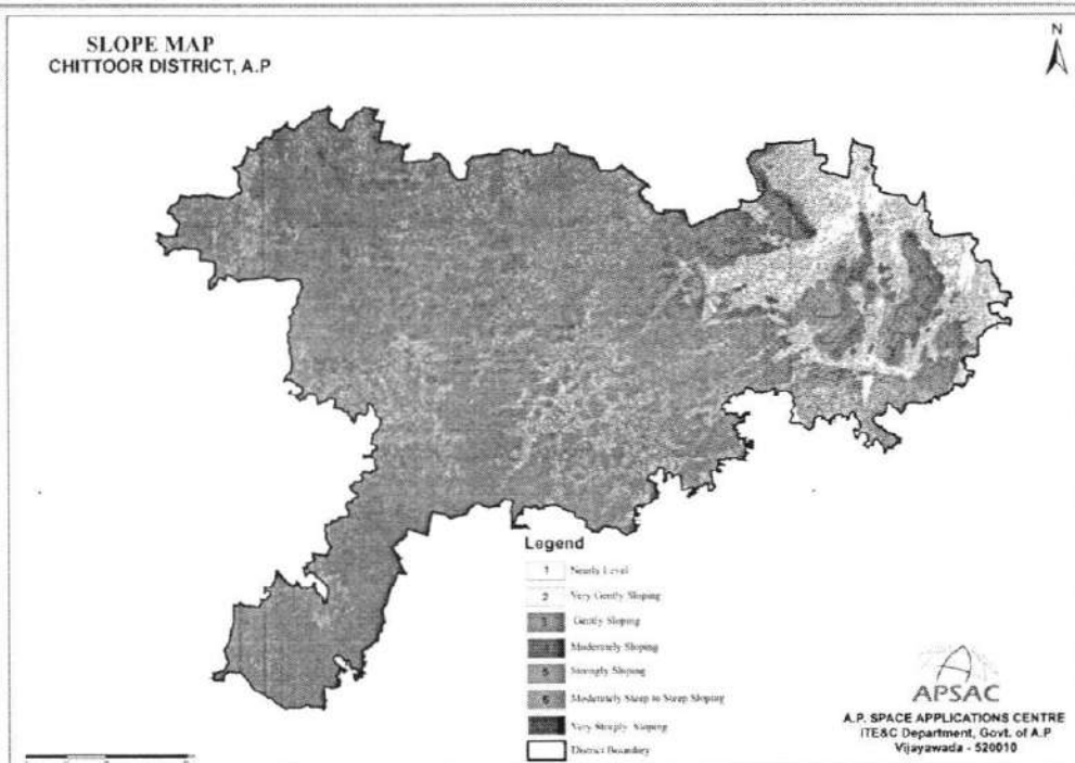
Fig:11 Slope map of chittoor district,A.P
