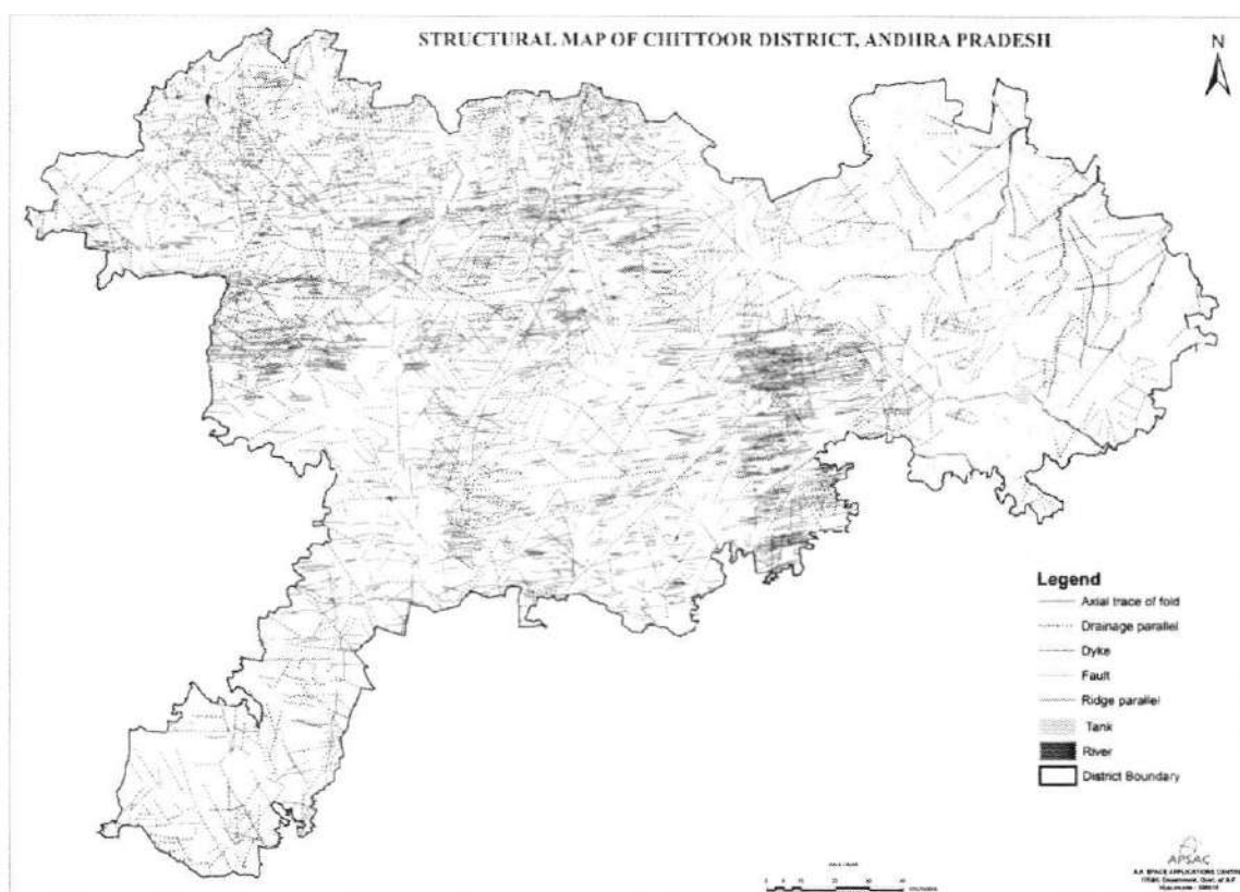
Structural Map of chittoor district, A.P
