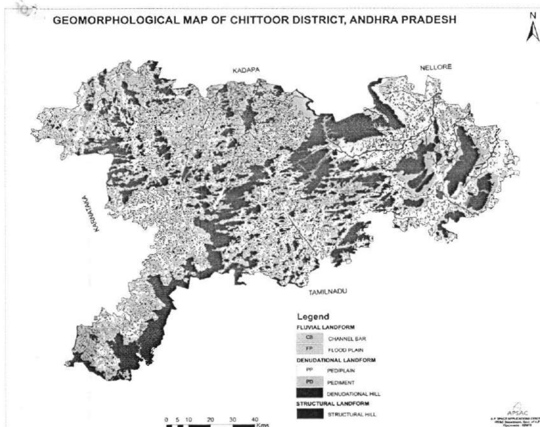
Fig 21:Geomorphological Map of Chittoor District,A.P
