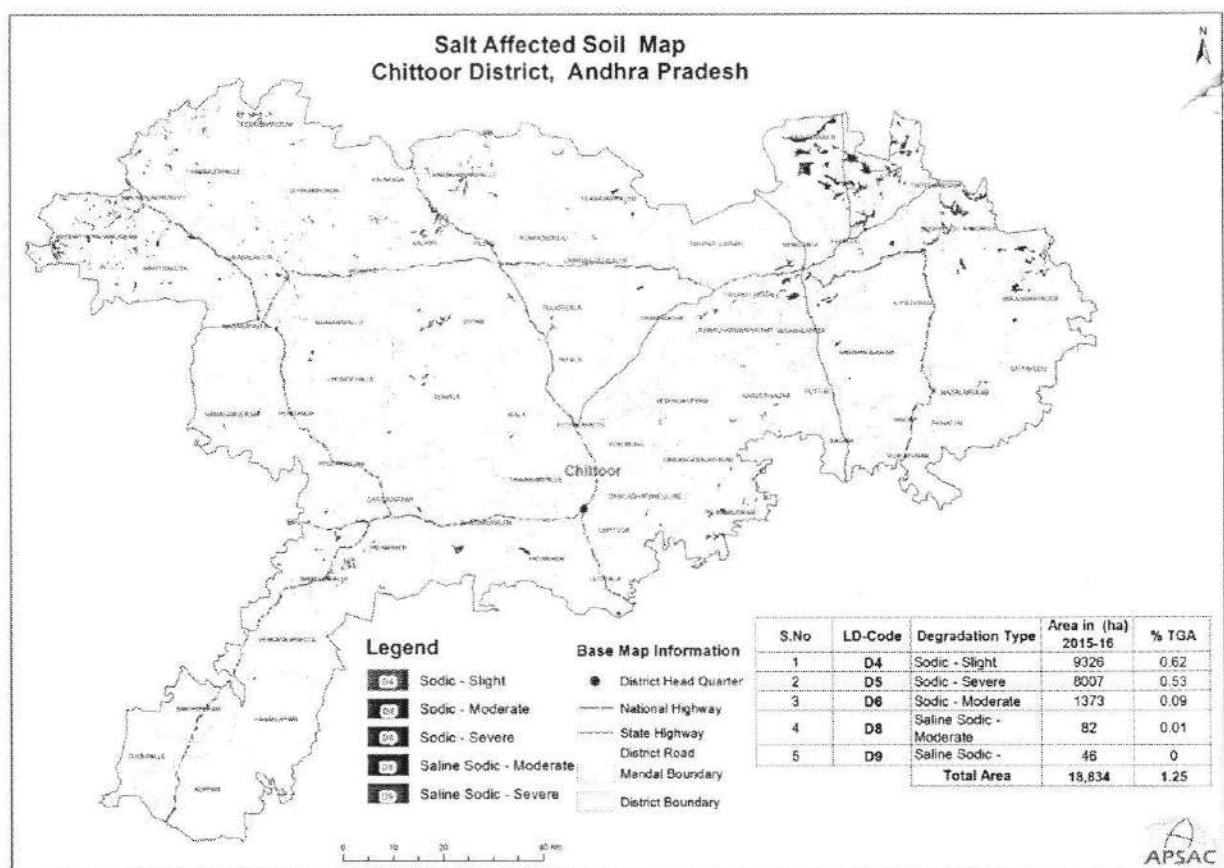
Fig.16, Salt affected land of Chittoor District,A.P
