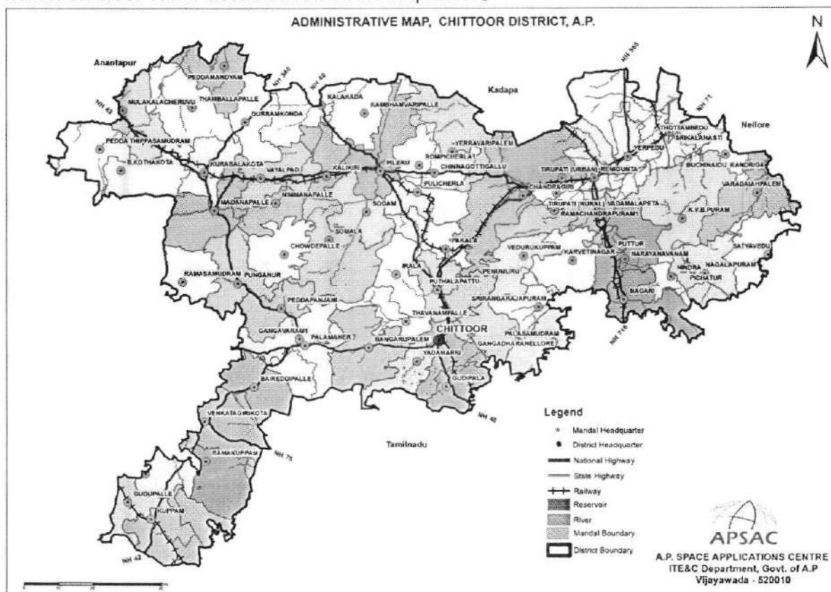
Fig.1 Administrative Boundaries of Chittoor District, Andhra Pradesh
