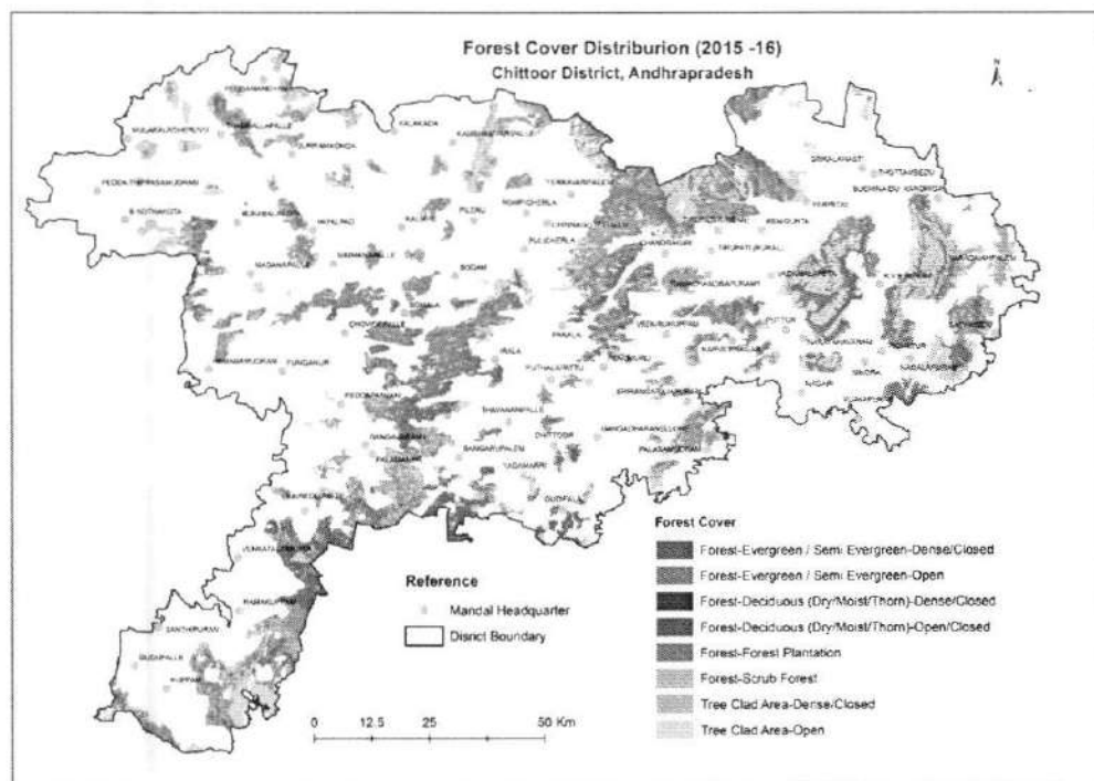
Fig:13 Forest cover map of Chittoor
