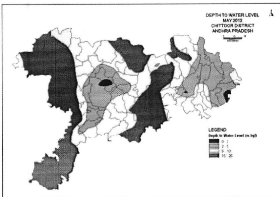
Fig.24. Premonsoon Water levels of Chittoor District.A.P
